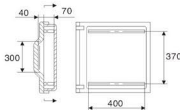
DZ-400/2E 单室真空包装机 SINGLE CHAMBER VACUUM PACKAGING MACHINE
