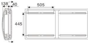
DZ-500/2SB
