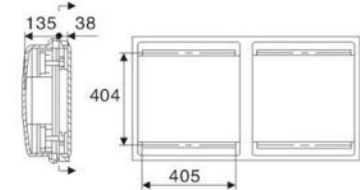
DZ-400/2SA
