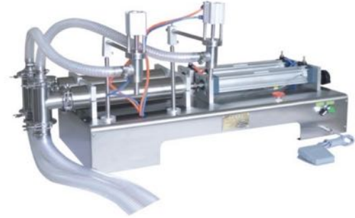
G2WY 双头液体灌装机 G2WY DOUBLE HEADS LIQUID FILING MACHINE
