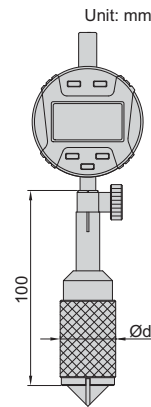
Unit: mm
