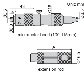
extension rod
